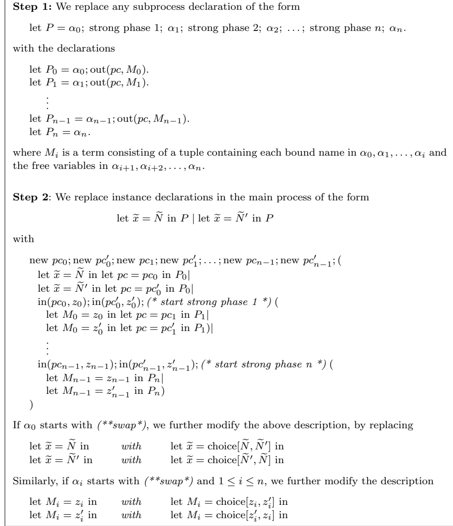
Fig. 1 Translator algorithm
